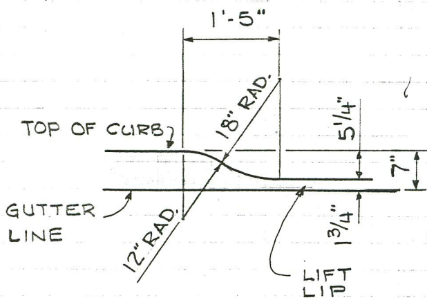
DETAIL
