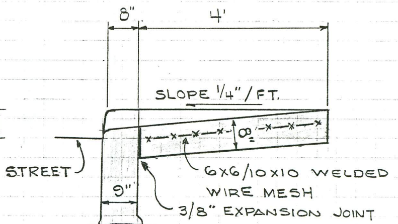
SECTION
